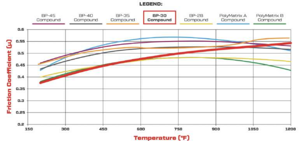
BP-30 Friction Coefficient and Temperature Values
